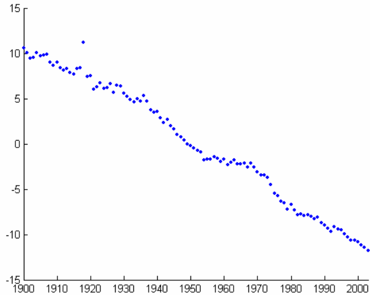
Figure 3.4: Dynamics of the Mortality Factor k_t from the Lee-Carter Model
