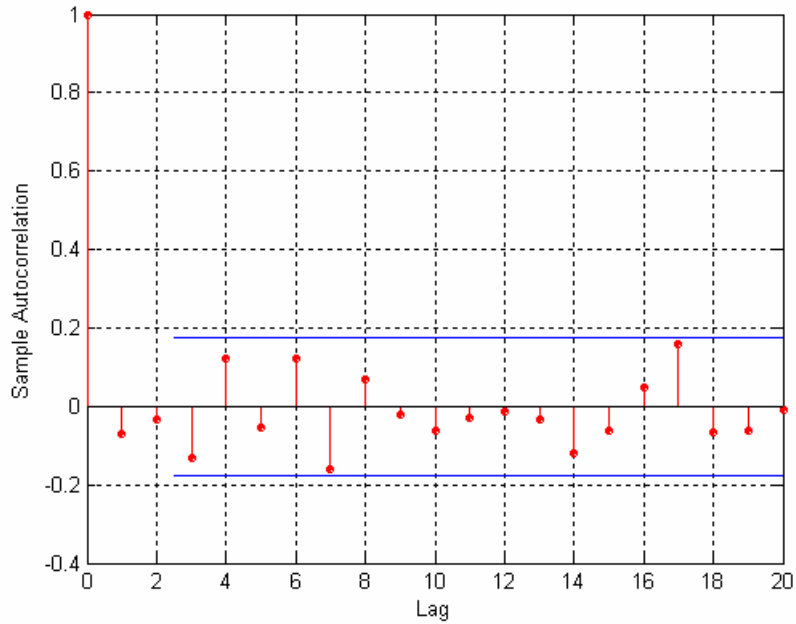
Figure 4.8: ACFs of Standardized Innovations of ARMA(2,0) + GARCH(1,1)
